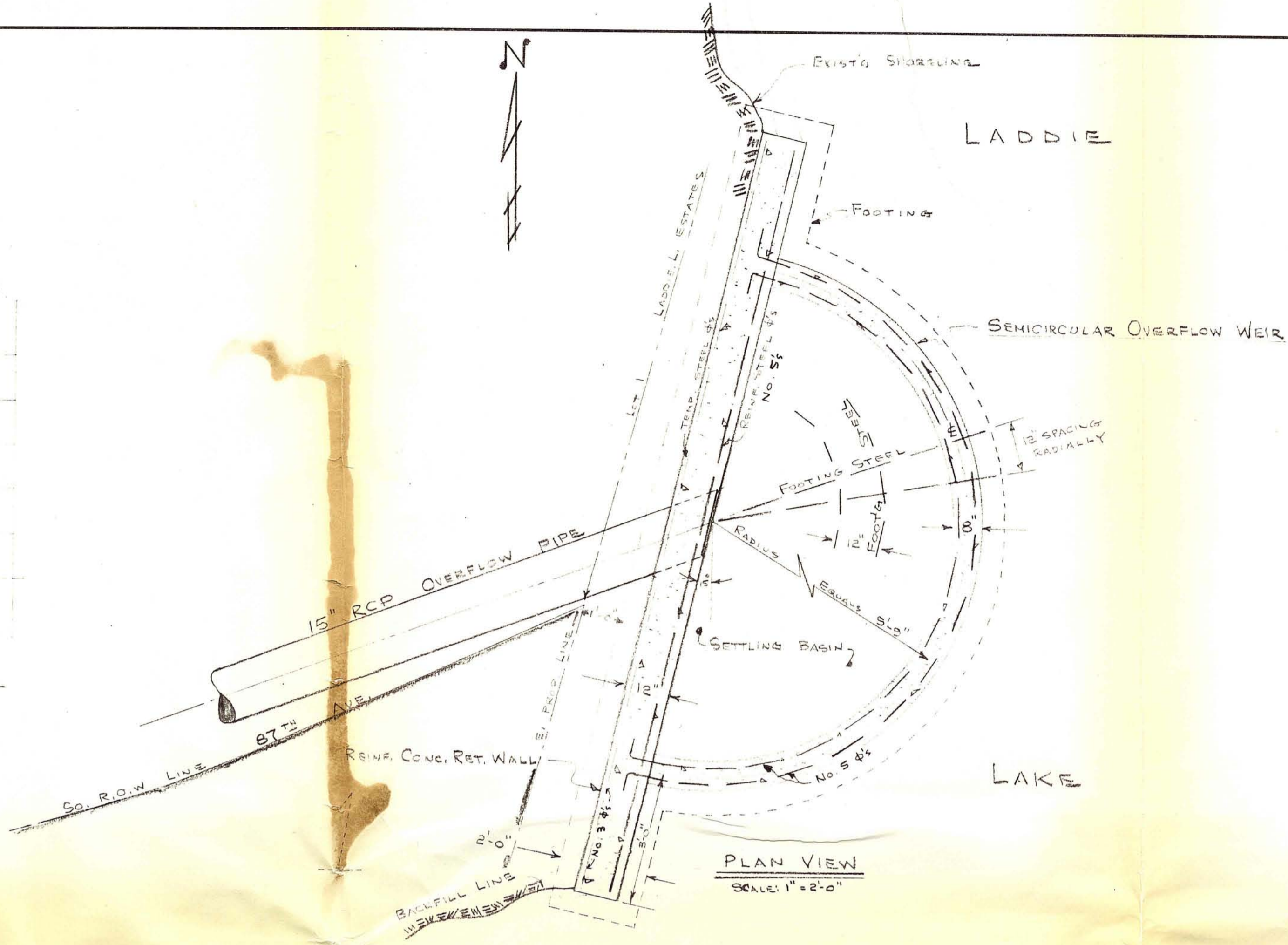
OVERFLOW CONTROL STRUCTURE
