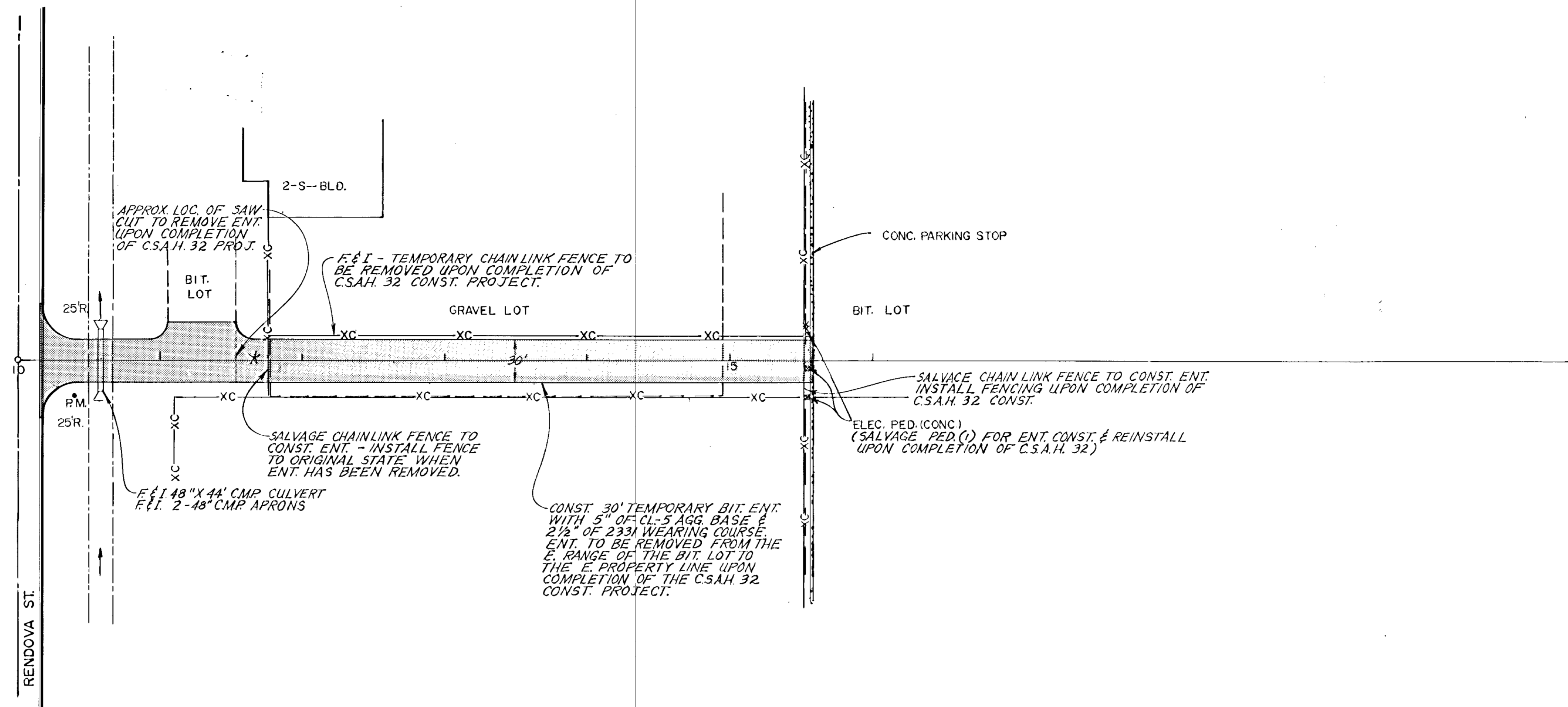
TEMPORARY ENTRANCE CONST. - RENDOVA ST. EAST
