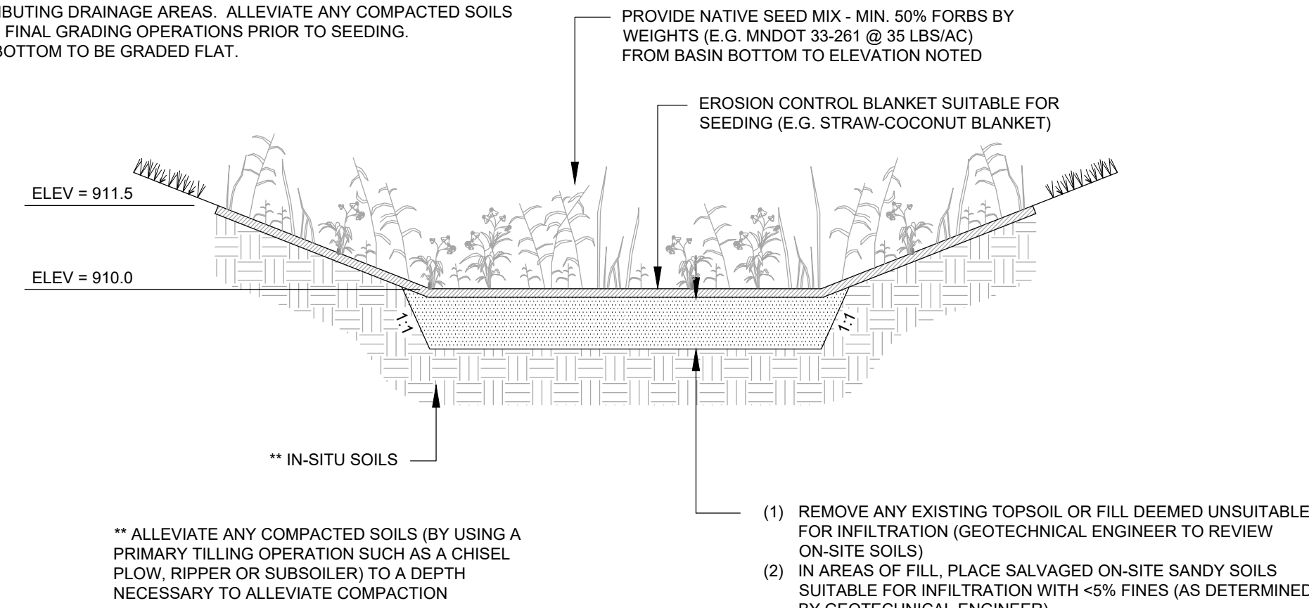
INFILTRATION BASIN N.T.S.
