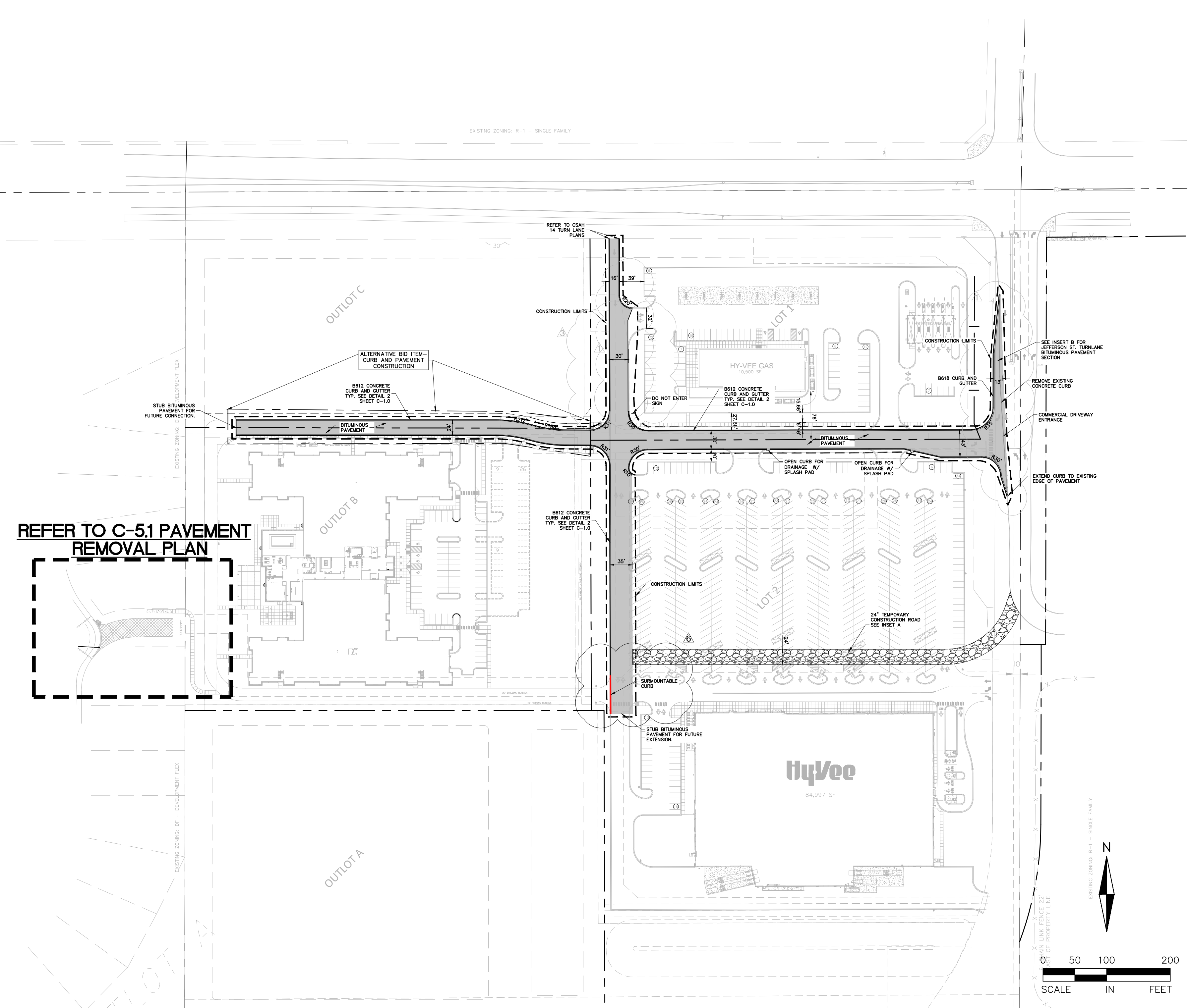
INSET A – TEMPORARY CONSTRUCTION ROAD
