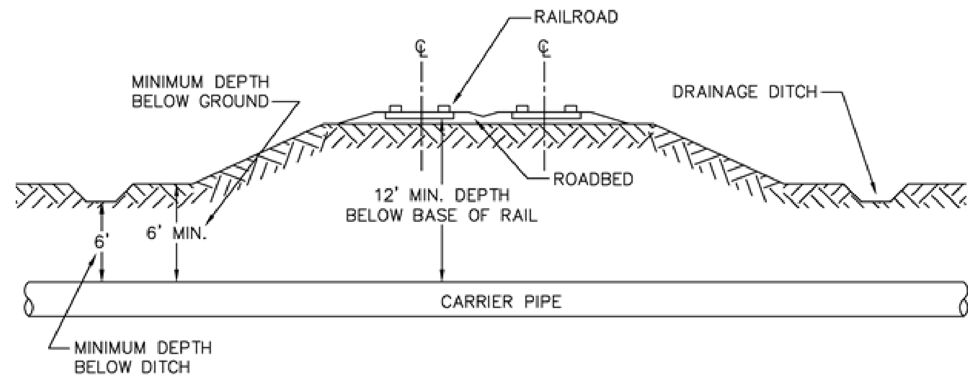
RAILROAD CROSSING (WITHOUT CASING)
