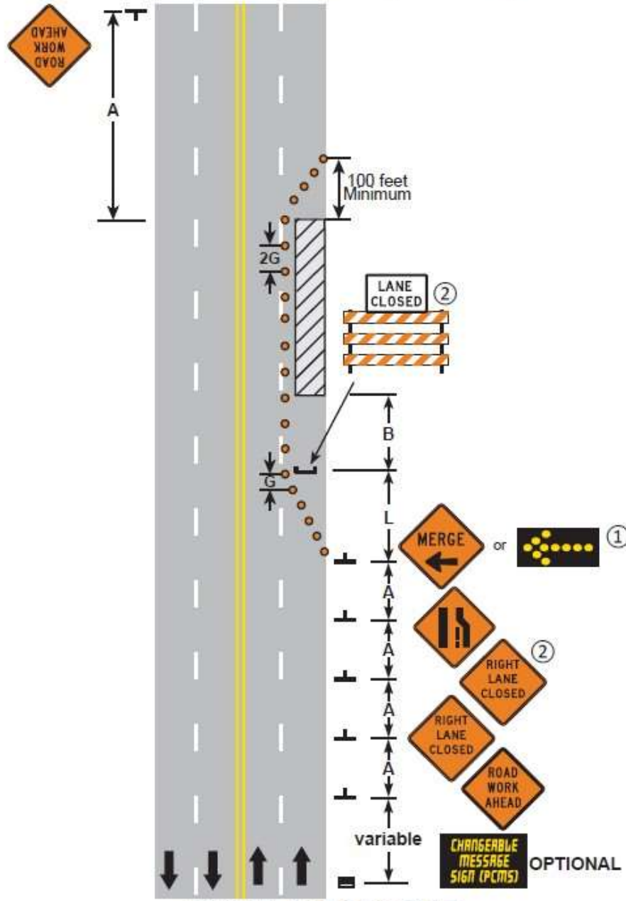
RIGHT LANE CLOSURE MULTI-LANE UNDIVIDED ROAD 3 DAYS or LESS LAYOUT 42 6K-42
