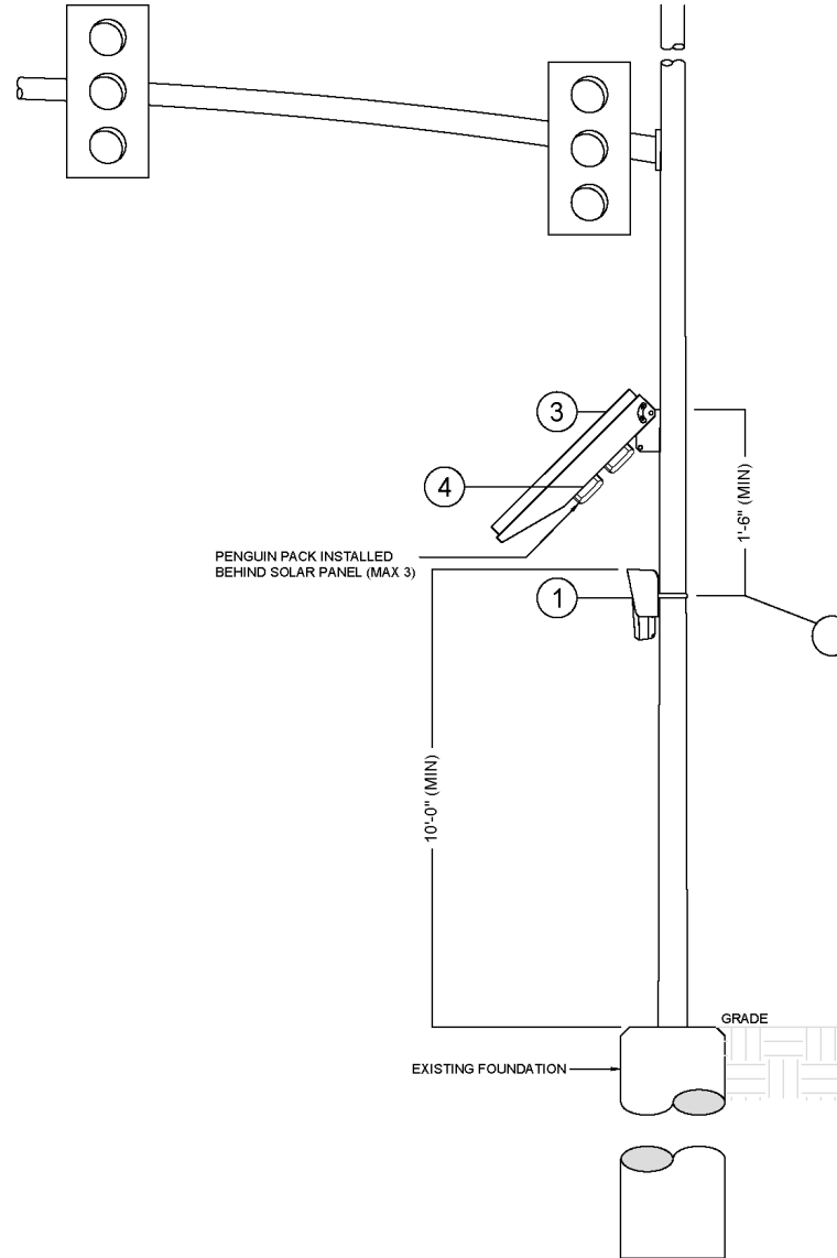
1 POLE ELEVATION DETAIL SCALE: N/A
