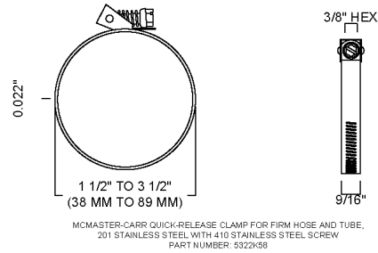
MOUNTING CLAMP
