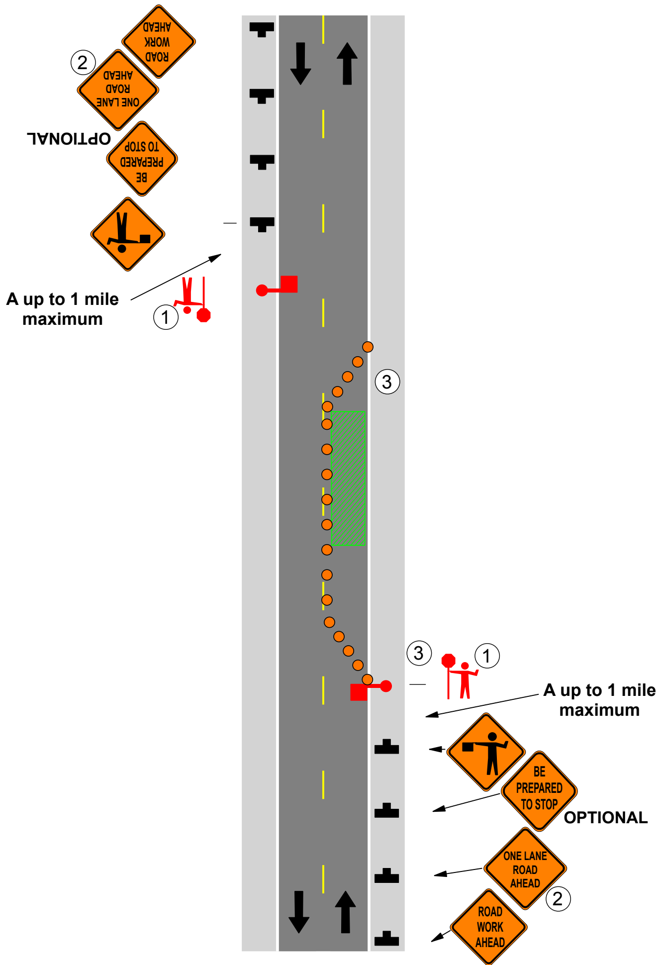
LANE CLOSURE, TWO FLAGGERS TWO-LANE, TWO-WAY ROAD
