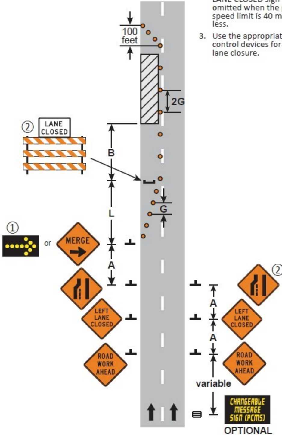
LANE CLOSURE MULTI-LANE DIVIDED ROAD
