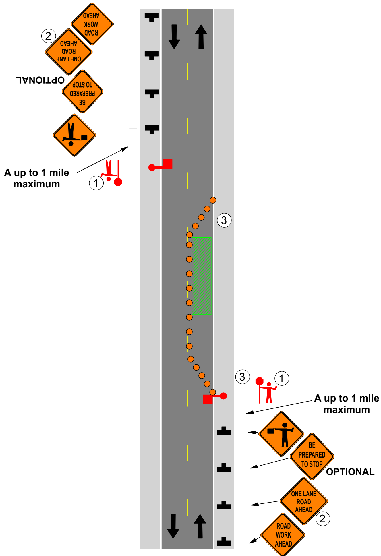
LANE CLOSURE, TWO FLAGGERS TWO-LANE, TWO-WAY ROAD
