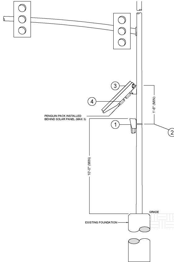
1 POLE ELEVATION DETAIL
