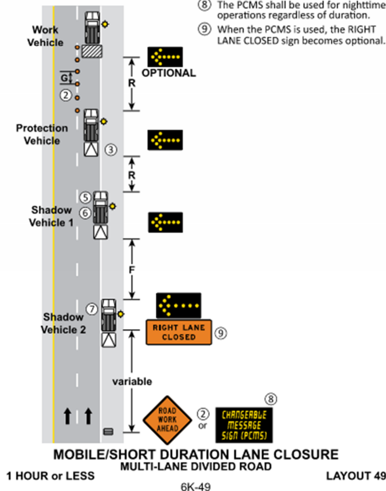
Figure 4: Multi-Lane Divided Road Mobile Traffic Control Plan, Source: MN MUTCD Part 6K, 2018
