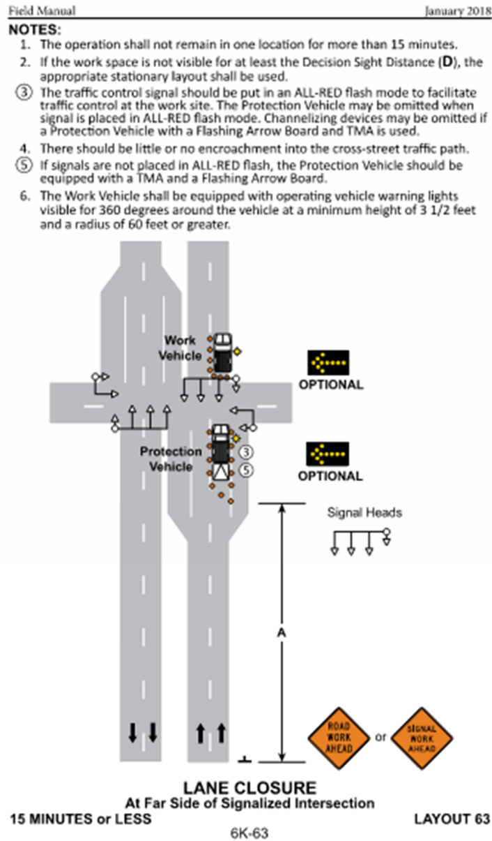
Figure 5: Lane Closure Near Intersection Traffic Control Plan, Source: MN MUTCD Part 6K, 2018
