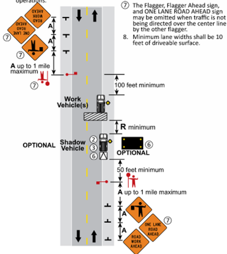
LANE CLOSURE With a Moving Work Area TWO-LANE, TWO-WAY ROAD 15 MINUTES or LESS LAYOUT 13 6K-13
