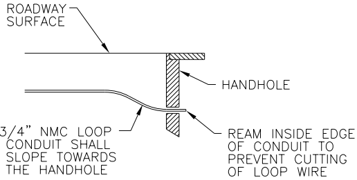
DRAINAGE DETAIL
