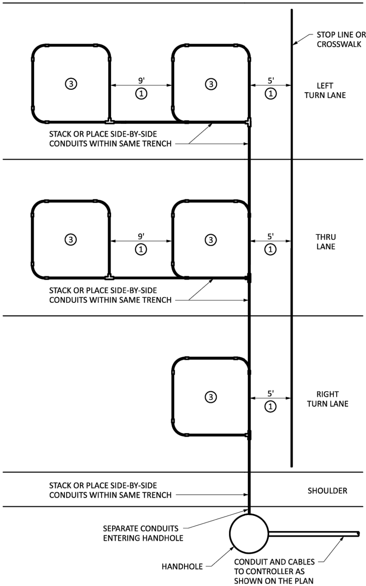
RIGID PVC LOOP DETECTOR PLACEMENT DETAIL
