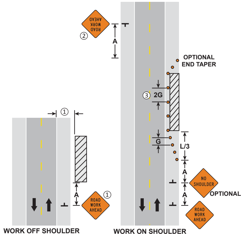
SHOULDER AND PARKING LANE CLOSURE Work On or Near Shoulder 3 DAYS or LESS LAYOUT 8 6K-8
