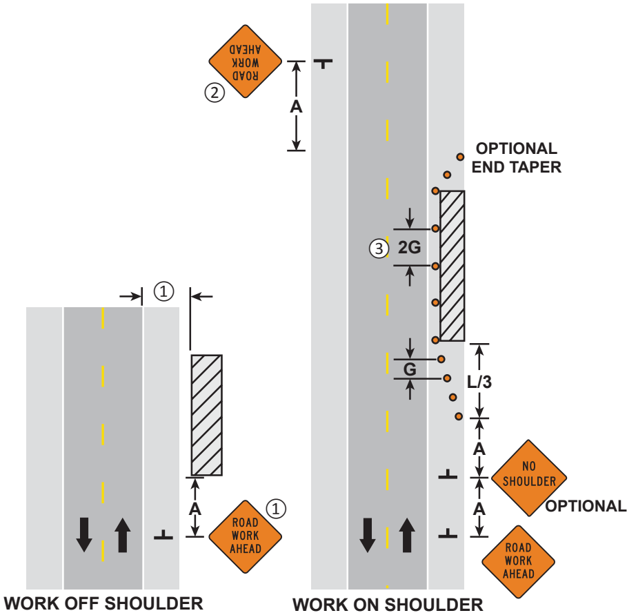
SHOULDER AND PARKING LANE CLOSURE Work On or Near Shoulder 3 DAYS or LESS 6K-8 LAYOUT 8
