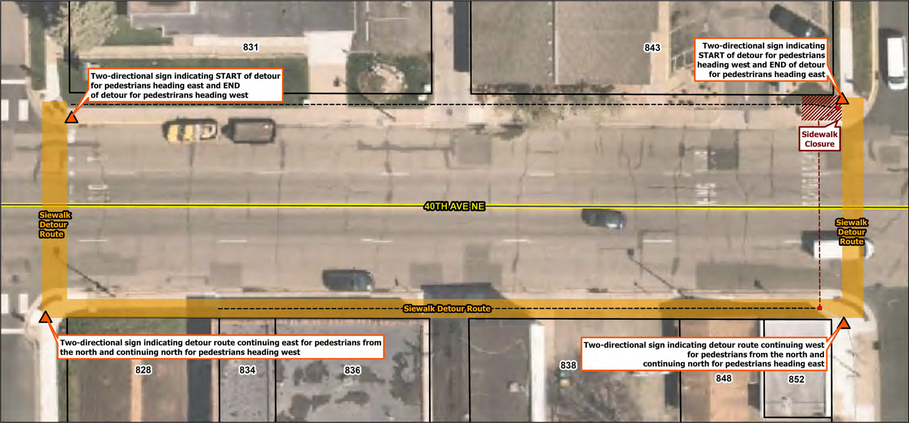
SIDEWALK CLOSURE PLAN
