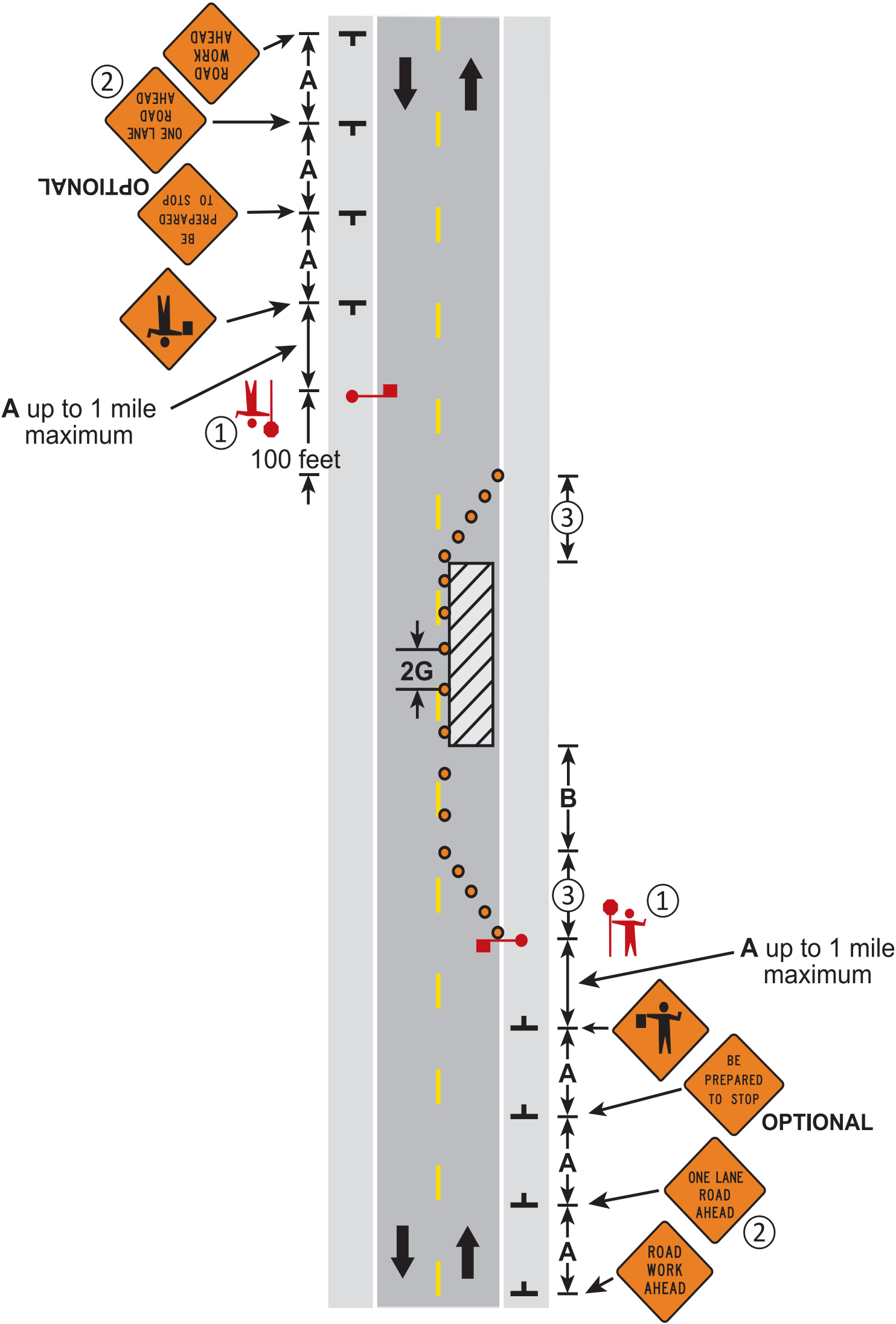
LANE CLOSURE, TWO FLAGGERS TWO-LANE, TWO-WAY ROAD
