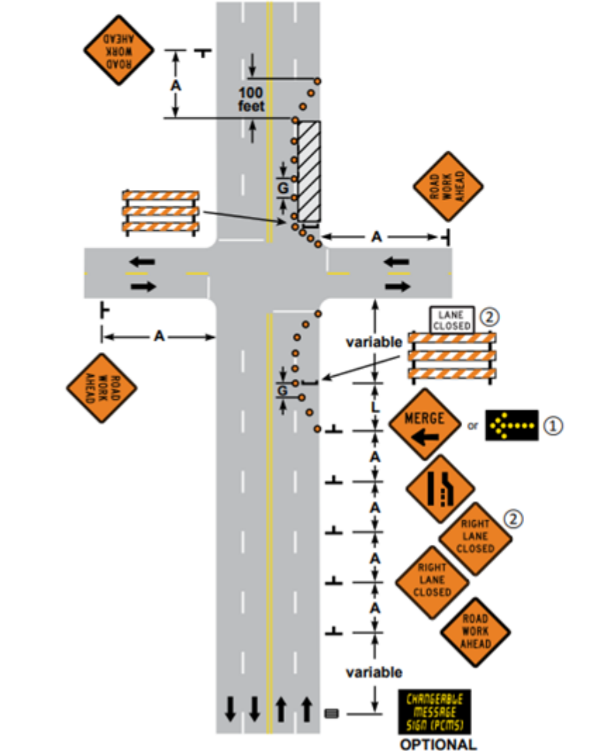
RIGHT LANE CLOSURE Work Space at Intersection MULTI-LANE UNDIVIDED ROAD 3 DAYS or LESS 6K-45 LAYOUT 45
