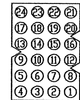
FRONT VIEW OF J1 HARNESS (SWITCH PANEL)
