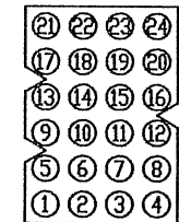
FRONT VIEW OF J1 JACK (SWITCH PANEL)
