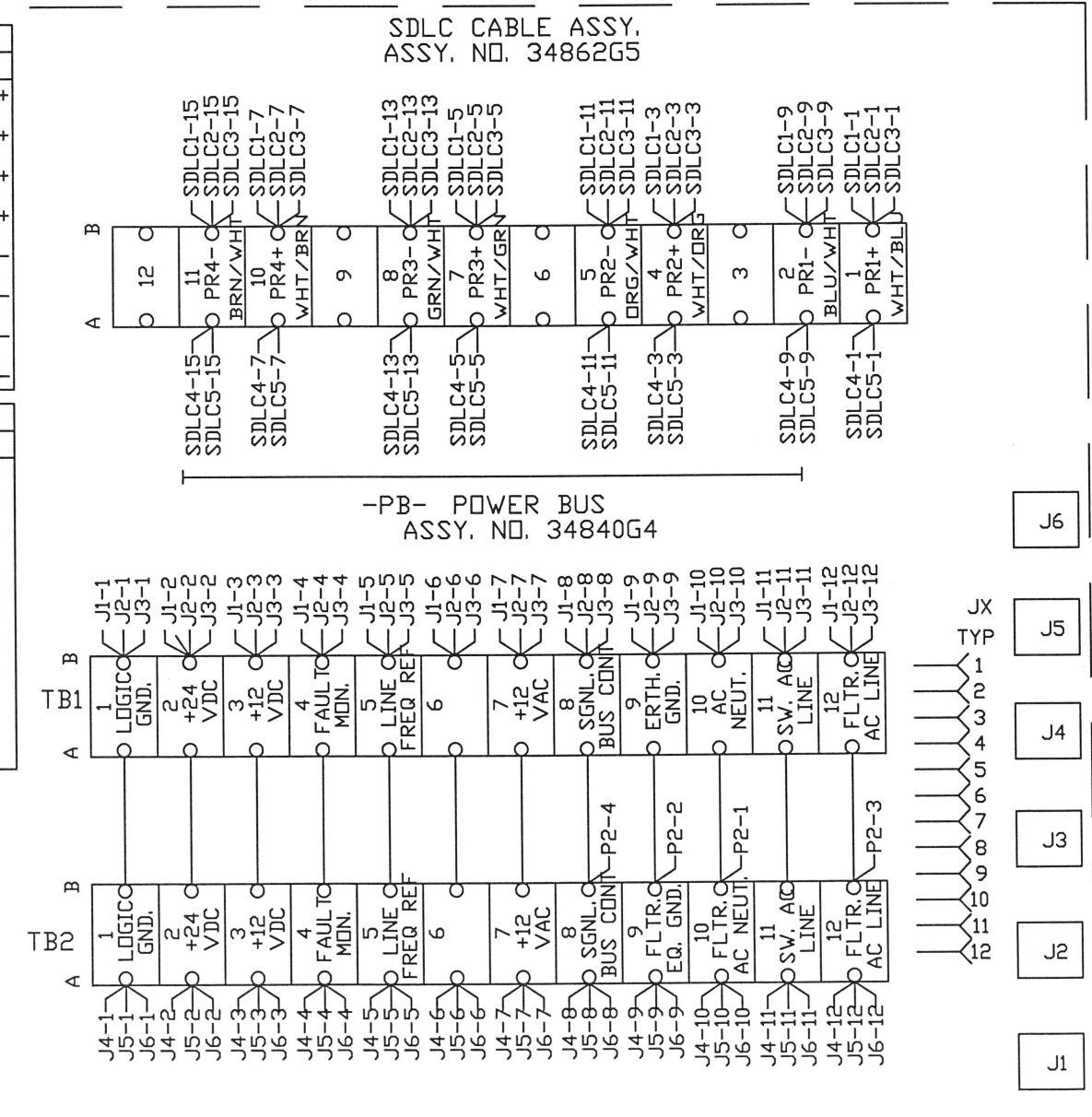
FRONT VIEW OF BU1 - BU5
