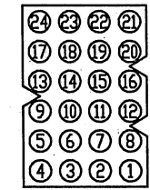
FRONT VIEW OF J1 HARNESS (SWITCH PANEL)
